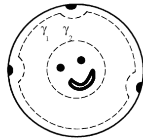
Figure 6. To find the conservation law for topological charges in the bounded volume, one uses two imaginary surfaces (dashed lines) to surround all the defects in the bulk and all the defects at the surface.
